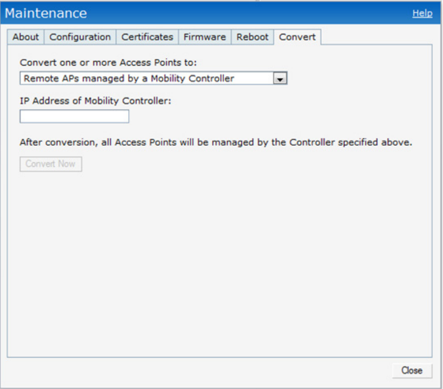
Figure 4 IAP-RAP Conversion over the Internet
