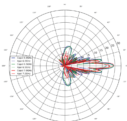
Azimuth, Vertical
