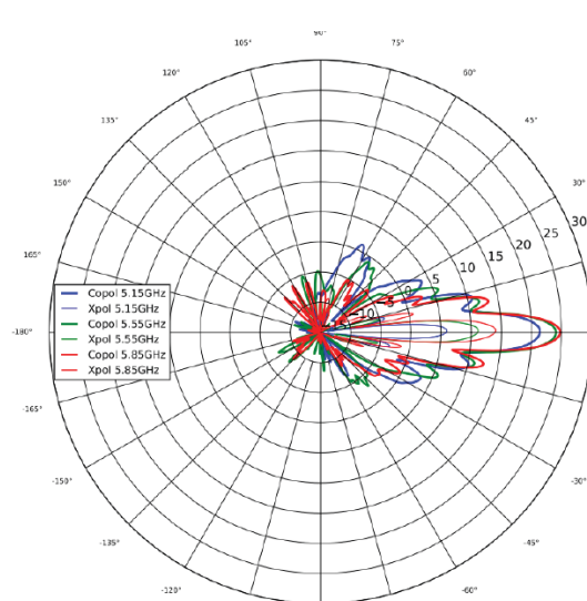
Elevation, Vertical
