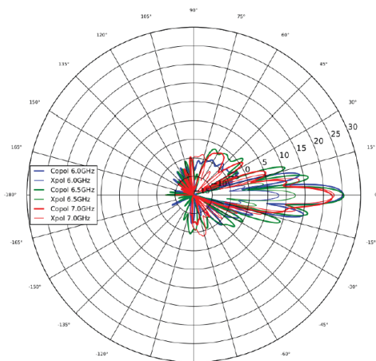
Azimuth, Horizontal
