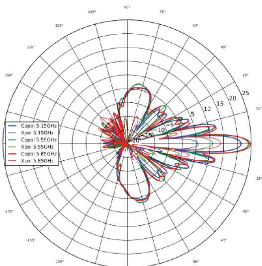
Azimuth, Vertical
