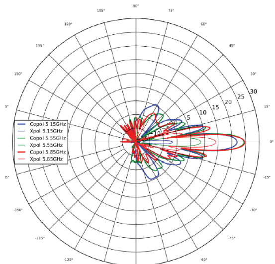
Azimuth, Horizontal
