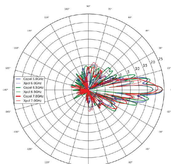
Elevation, Vertical
