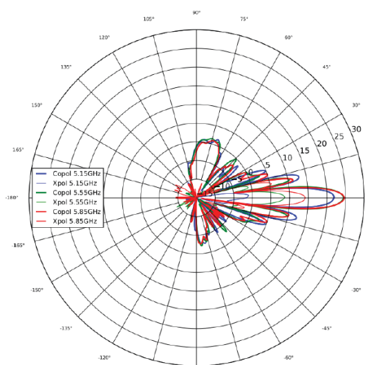
Elevation, Horizontal
